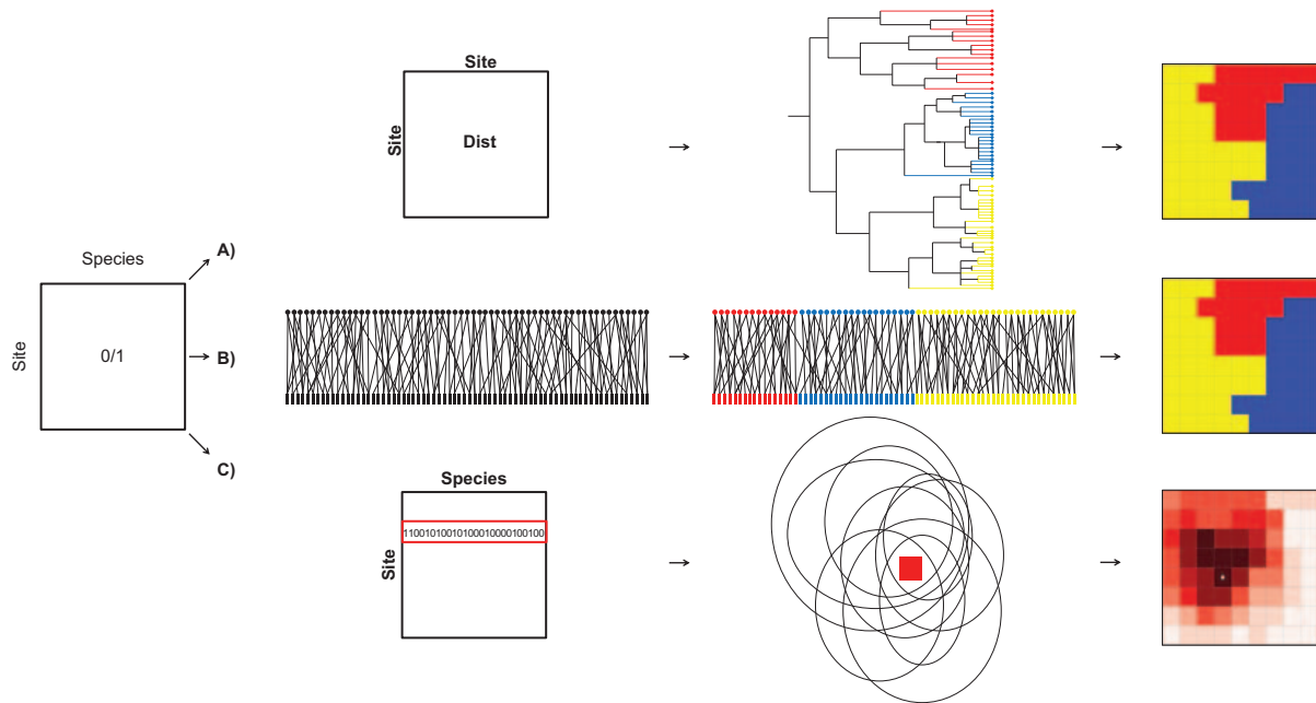
Figure 1. Schematic overview of three approaches to define the biogeographic species pool. (A) Distance-based clustering analysis. The first step of a clustering analysis is calculating the distance between sites (in this case grid cells) according to the similarity of their species assemblages. Similar sites are then classified into groups using a clustering algorithm. The appropriate number of groups is decided upon according to the results of the clustering analysis. The final result is the division of sites into biogeographic regions based on similarities of species assemblages across sites. (B) Network modularity analysis of species assemblages. First, species and sites are arranged as a two-mode (or bipartite) network, with sites (rectangles) and species (circles) sharing a link if the species is present at the site. Sites and species that are strongly interconnected are then grouped using a modularity analysis. The final result is conceptually the same as for clustering analysis; the division of sites into biogeographic regions based on site similarity. (C) Assemblage dispersion fields (ADFs). The ADF approach is site-specific. Sites can thus be included in the regionalization, or species pool, if they share at least one species with the focal assemblage. The ADF of a site is created by overlapping the geographic ranges of all the species occurring in the focal site, creating a site-specific species richness map. The colour intensity of a cell indicates the height of the ADF, that is, darker cells share more species with the focal cell. The focal cell is marked by a white dot.
